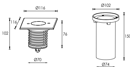
Mounting sleeve 015#
